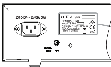
Rear view of Central unit
